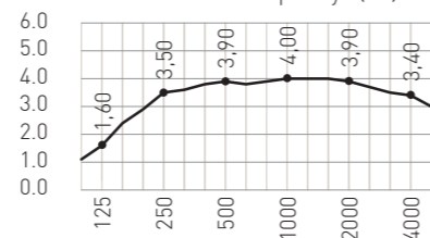
Absorption area A_{\text{obj}} /m 2 at one-third centre frequency f (Hz)
