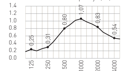
Sound absorption coefficient \alpha_w at one-third centre frequency f (Hz)
